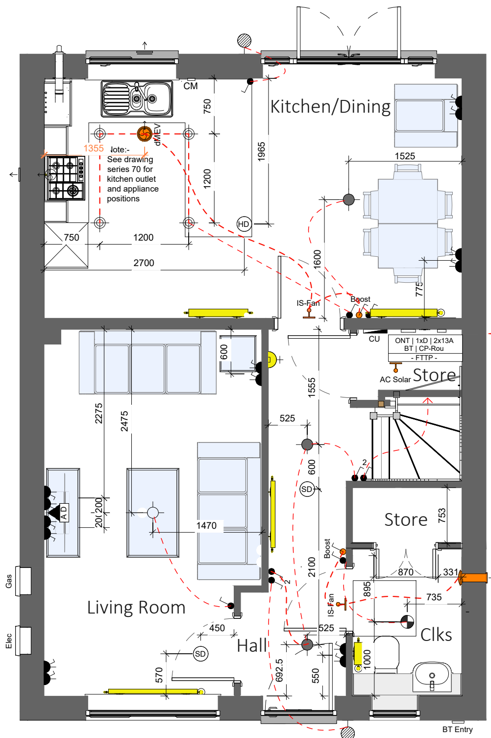
1 Ground Floor Electrical GA 1 : 50
