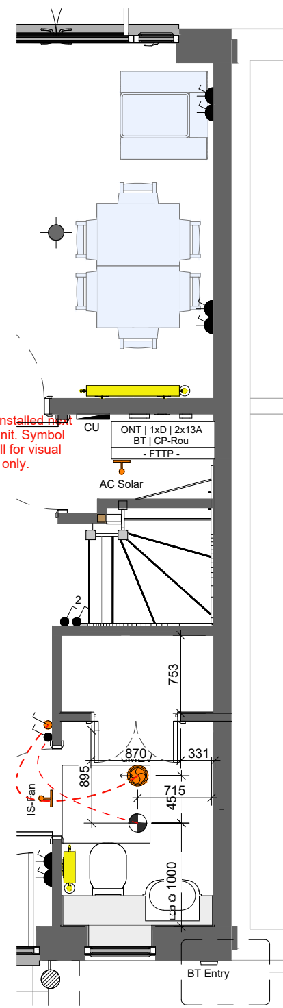
2 Ground Floor - Semi-Detached Callout 1 : 50 Plots 08, 14, 50 (AS) & 01, 03, 09, 18, 19, 49 OPP
