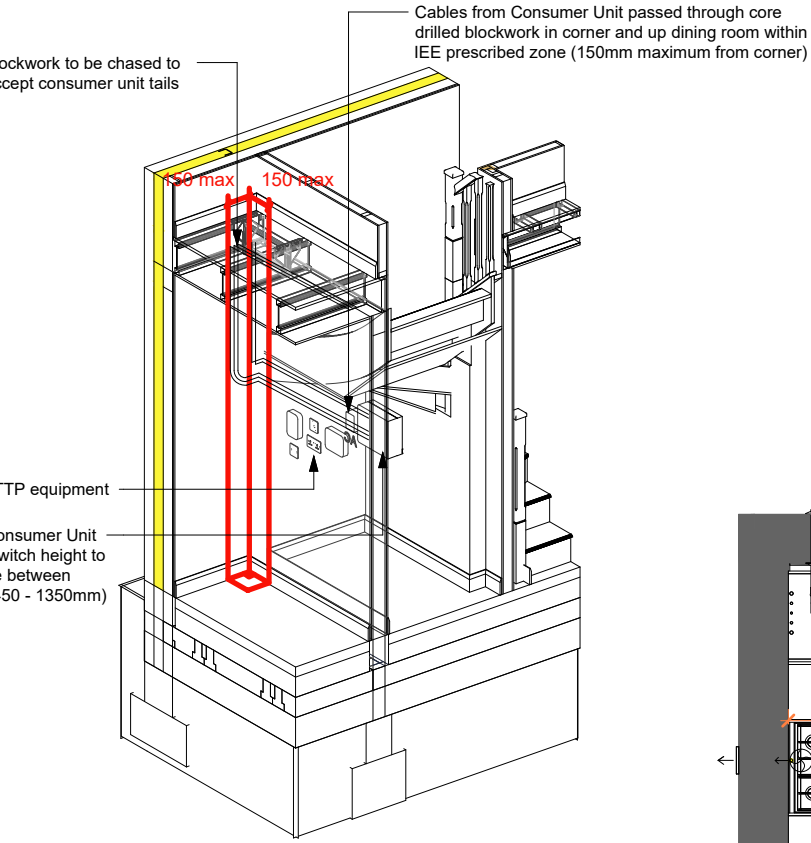
3 AT Understair Cupboard
